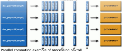
Parallel computing example of processing payroll
